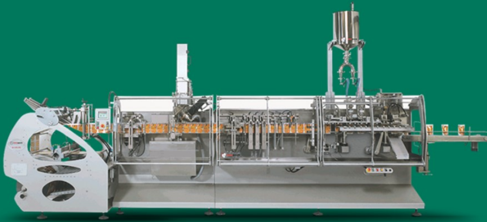
HORIZONTAL FORM FILL SEAL
